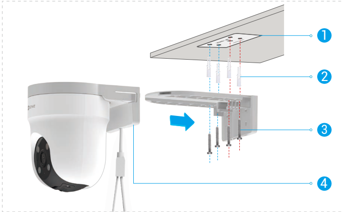
Fig. 1 Ceiling Mount
