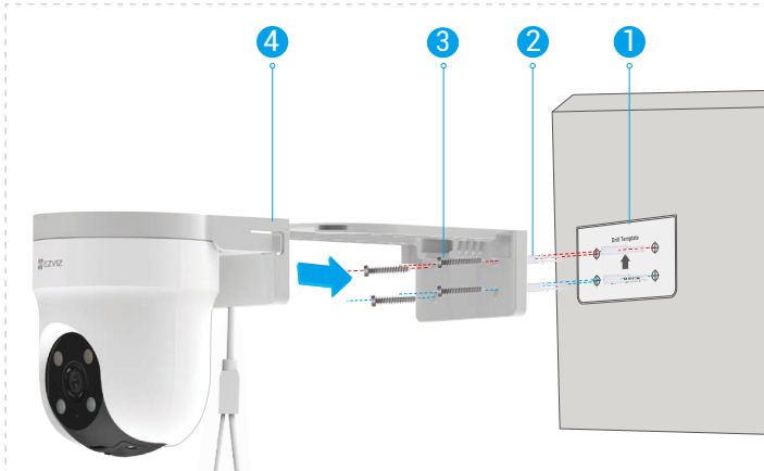
Fig. 2 Wall Mount
